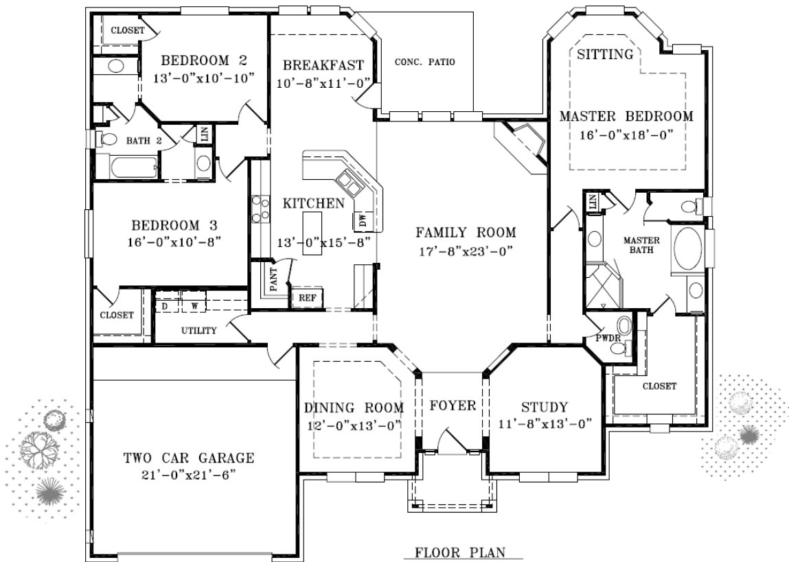
FLOOR PLAN
